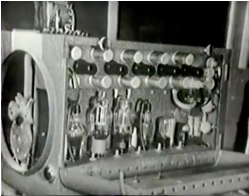
Camera, showing location of the color wheel
