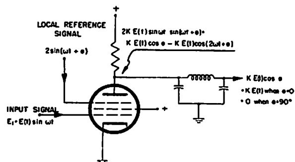
Fig. 9 - Principle of Synchronous Demodulation
