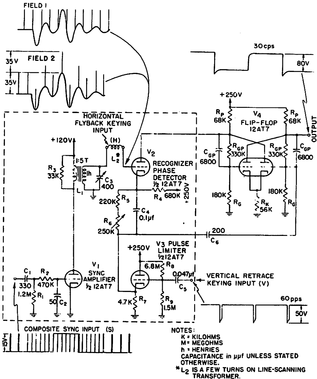
Fig. 12 - Field Recognition Circuit for Color Phase Alternation
