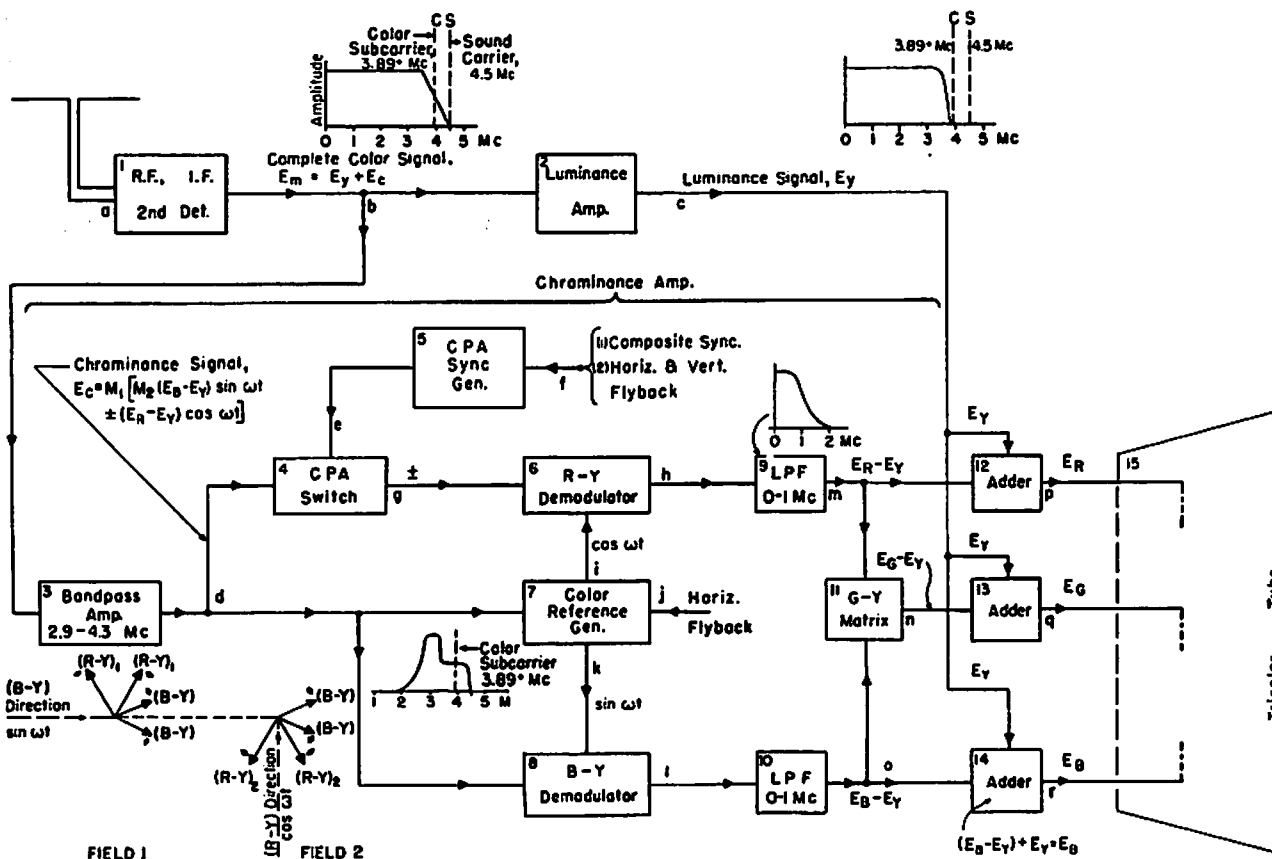
Fig. 3 - Block Diagram of a Color Receiver
