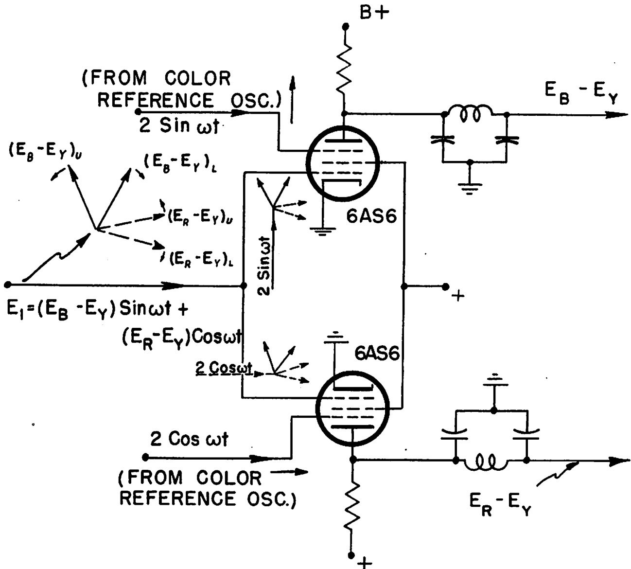
Fig. 10 - Quadrature Demodulation
