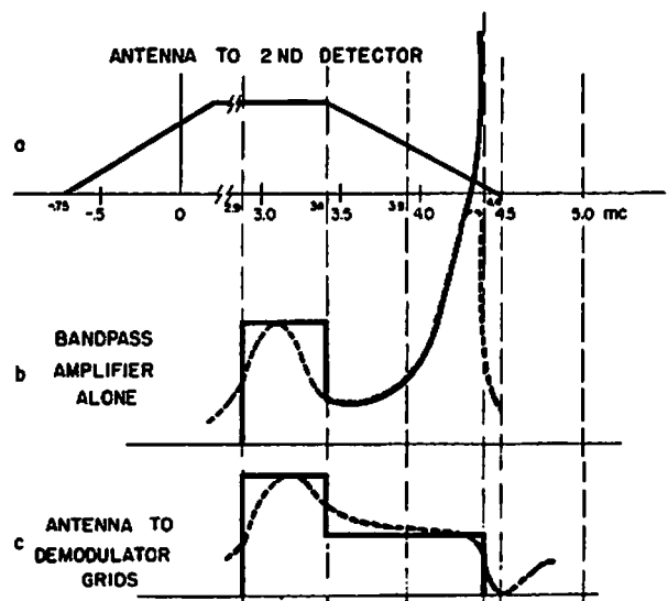
Fig. 8 - Practical Approximation to Characteristic of Fig. 6b
