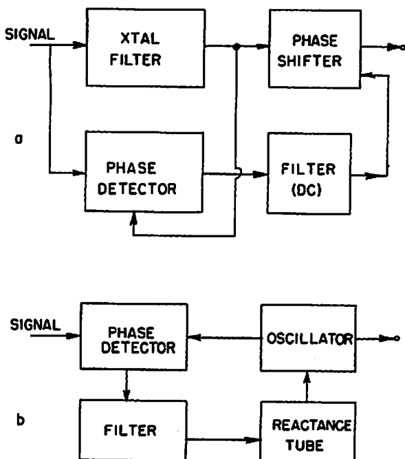
Fig. 11 - Practical Integrators for Color Reference Signal
