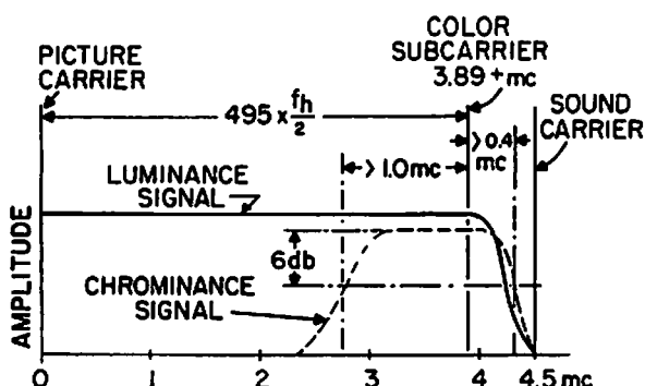
Fig. 1 - Spectrum of Complete Color Signal
