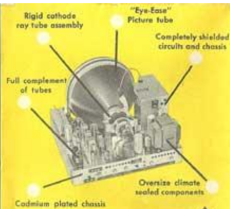
ILLUSTRATED 12 1/2-INCH TUBE CHASSIS
