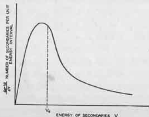
Fig. 10—Energy distribution of secondary electrons.
