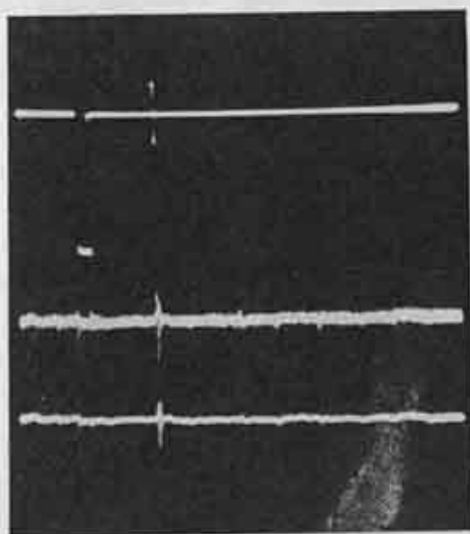
Fig. 8—Top line: Synthetic input signals used in tests. Variable signal is a pulse exactly like the steady pulse, but varying in amplitude from scan to scan. Middle line: Output without filter. Bottom line: Output filtered. Signals are in the same phase in each oscillogram.
