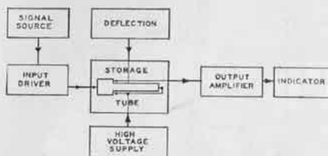
Fig. 1—Block diagram of storage tube cancellation circuits.
