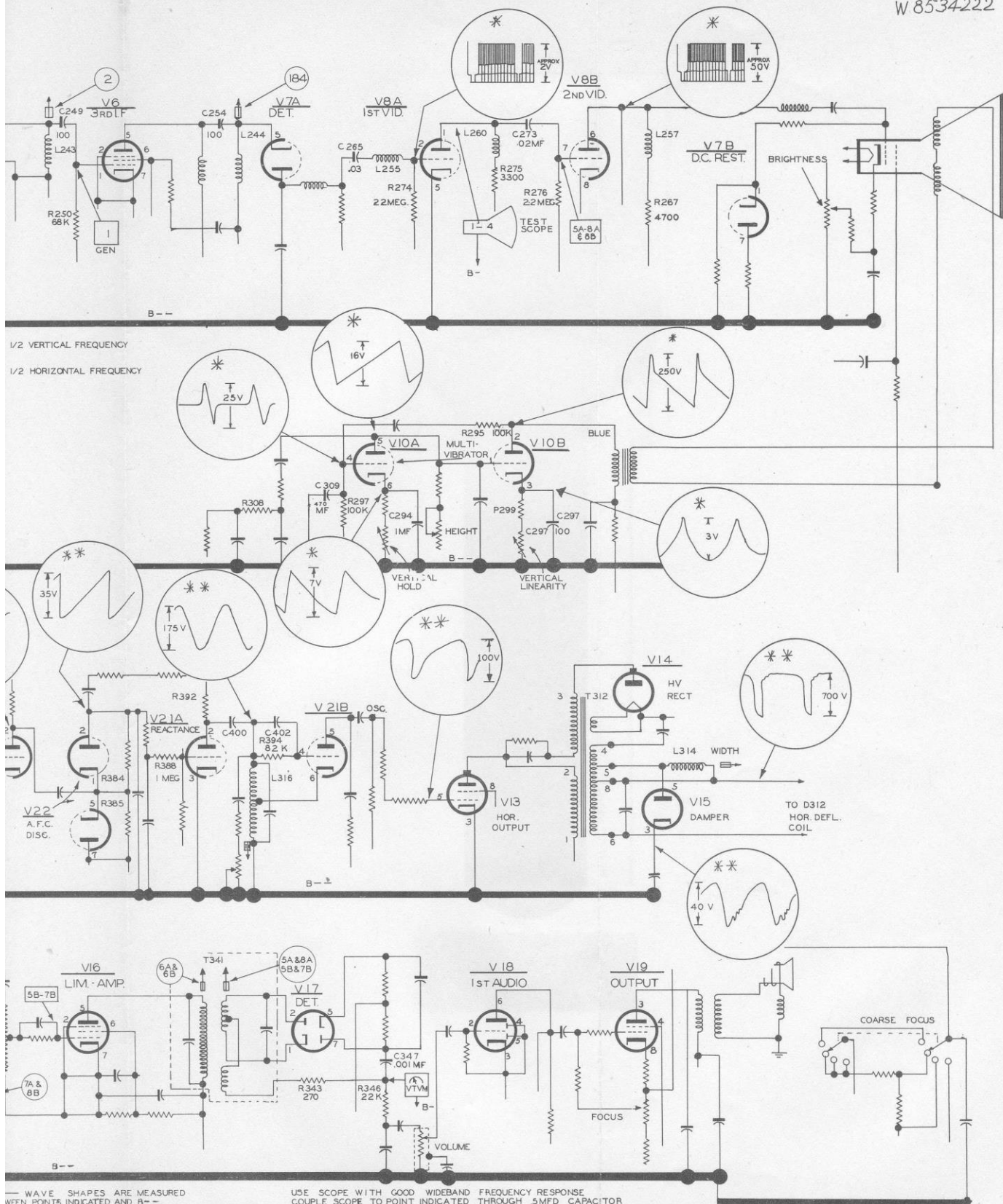
MODELS C-2505A, C-2506, & C-2509 Television Receivers Waveform Drawing
