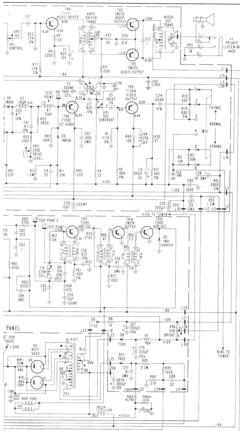
Schematic Diagram Courtesy of Philco Corporation
