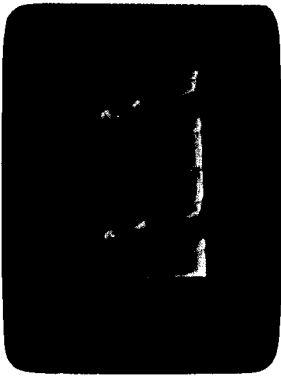
Figure 28 Description: Video + Sync Taken at: Pin 7 (grid) of 12AU7, DC restorer Oscilloscope Sweep Freq.: \frac{1}{2} H Peak-to-peak Voltage: Video, 27 Video + Sync, 36
