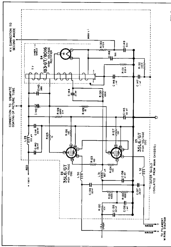
Figure 14. Schematic of High-Voltage Power Supply
