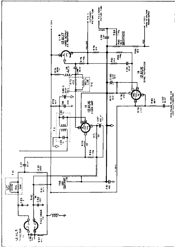
Figure 9. Video Amplifier and Sync Separator
